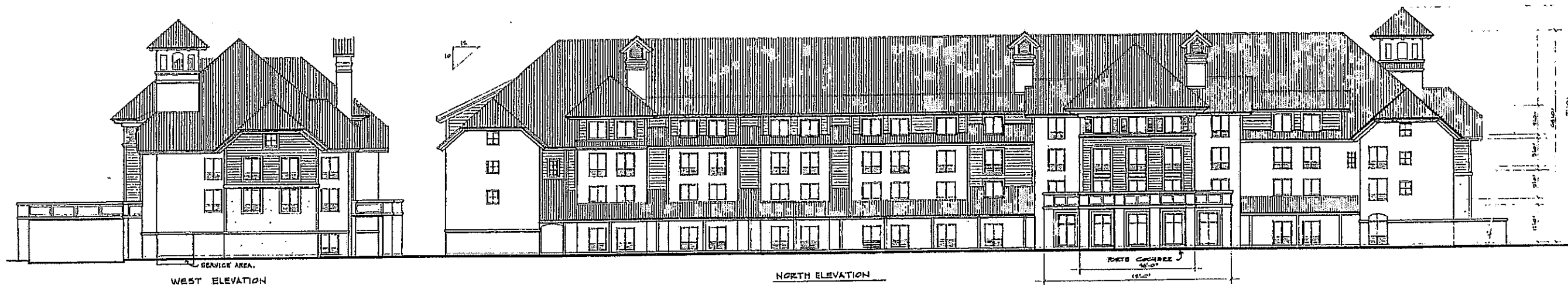
HOTEL BUILDING EXTERIOR ELEVATIONS
